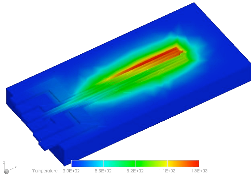
Profile of heat dissipated from the Gripper to the surrounding air
