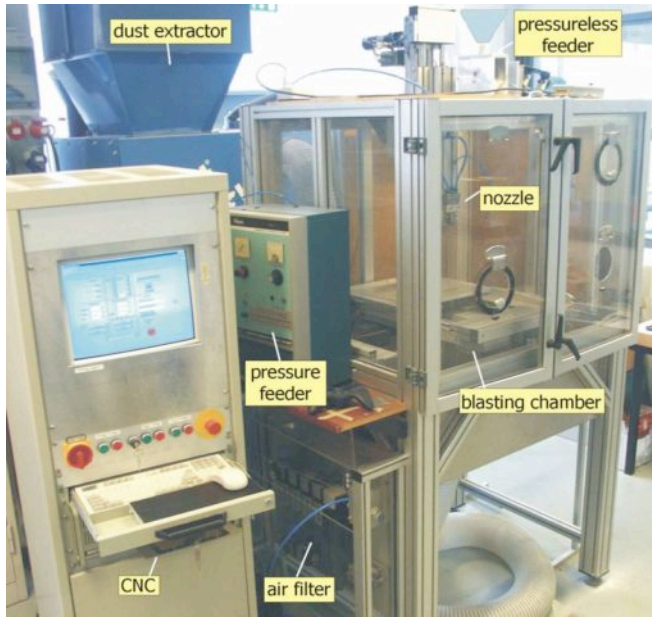
Abrasive blasting set up
